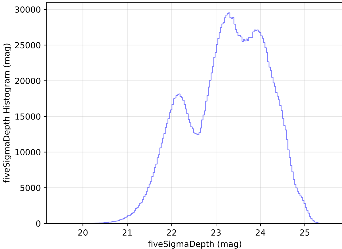
too_elab_r16_d2_griz_v3.4_10yrs WFD all bands: fiveSigmaDepth Histogram
