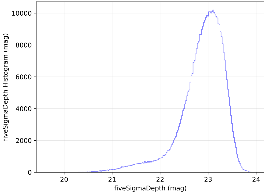
too_elab_r16_d2_griz_v3.4_10yrs All sky z band: fiveSigmaDepth Histogram
