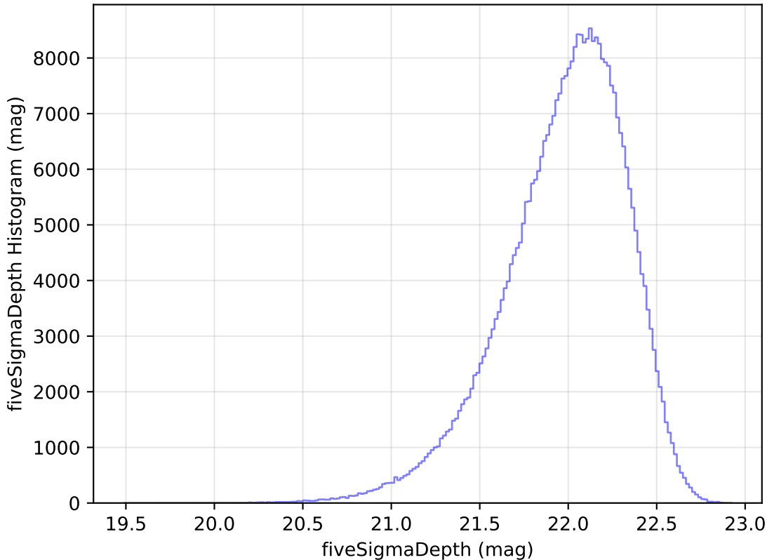
too_elab_r16_d2_griz_v3.4_10yrs All sky y band: fiveSigmaDepth Histogram
