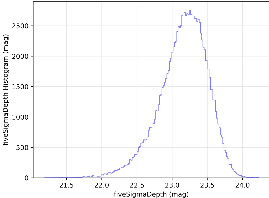
too_elab_r16_d2_griz_v3.4_10yrs All sky u band: fiveSigmaDepth Histogram
