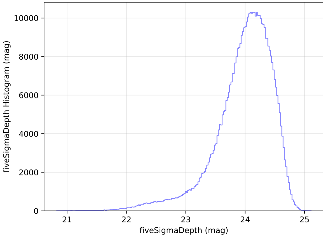
too_elab_r16_d2_griz_v3.4_10yrs All sky r band: fiveSigmaDepth Histogram
