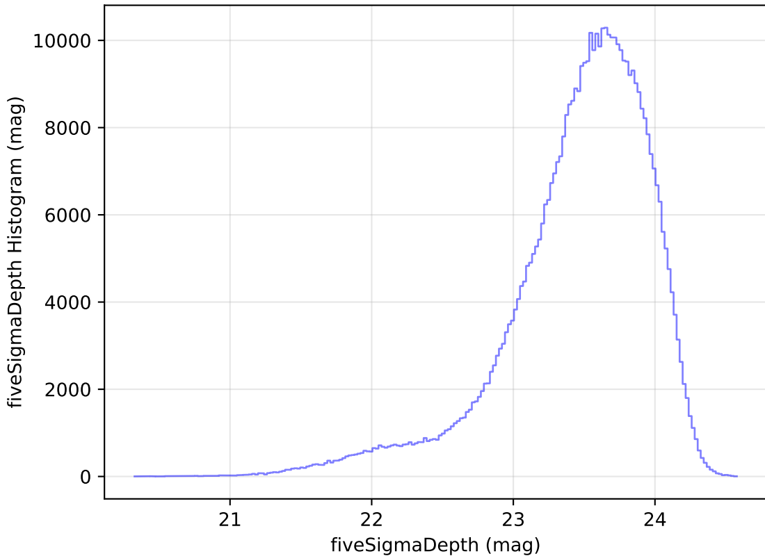
too_elab_r16_d2_griz_v3.4_10yrs All sky i band: fiveSigmaDepth Histogram
