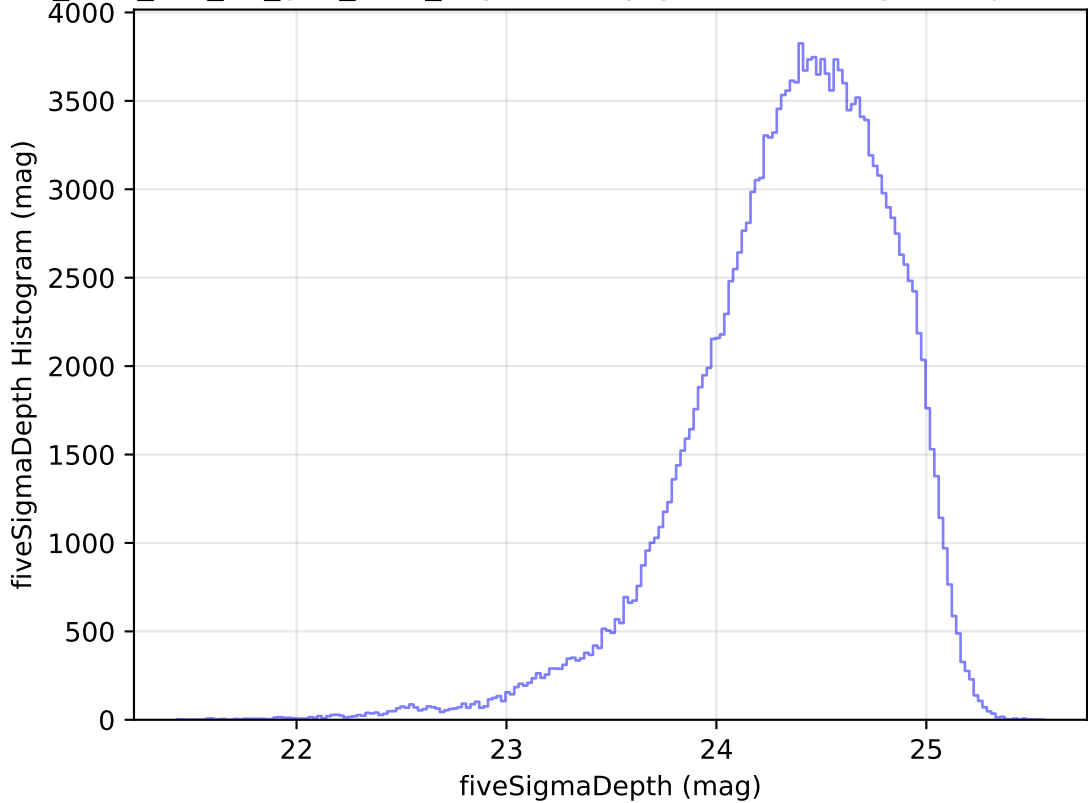
too_elab_r16_d2_griz_v3.4_10yrs All sky g band: fiveSigmaDepth Histogram
