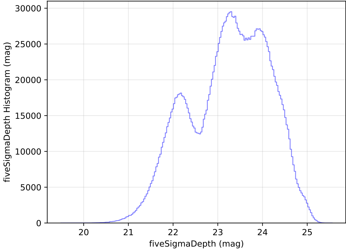
too_elab_r16_d2_griz_v3.4_10yrs All sky all bands: fiveSigmaDepth Histogram
