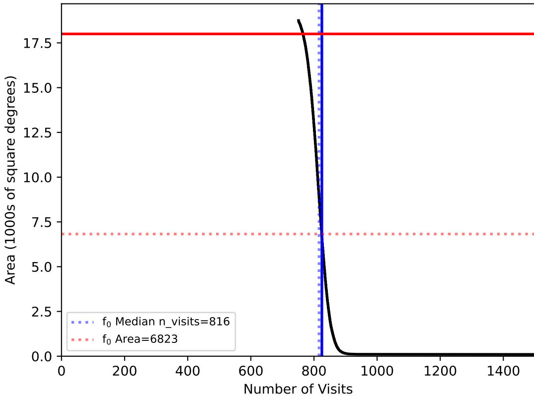
too_elab_r16_d2_griz_v3.4_10yrs WFD: fO
