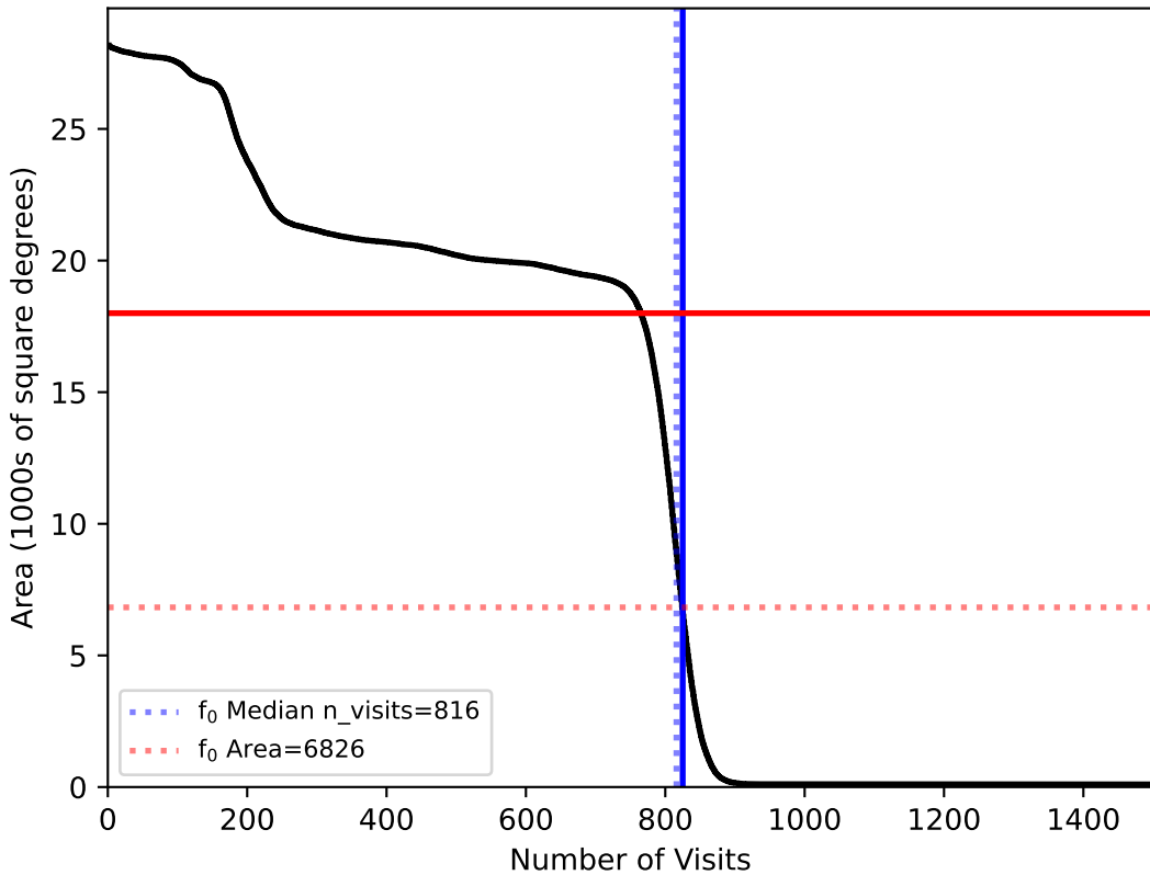
too_elab_r16_d2_griz_v3.4_10yrs All sky: fO
