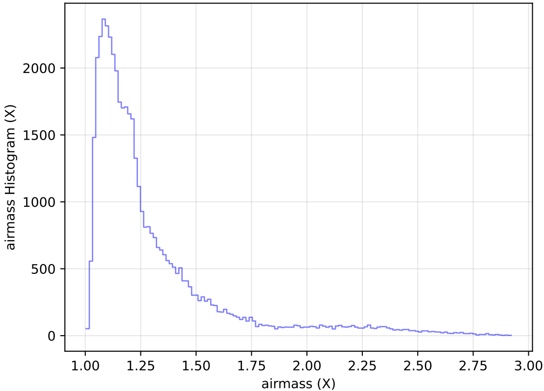
too_elab_r16_d2_griz_v3.4_10yrs Yr 1 z band: airmass Histogram
