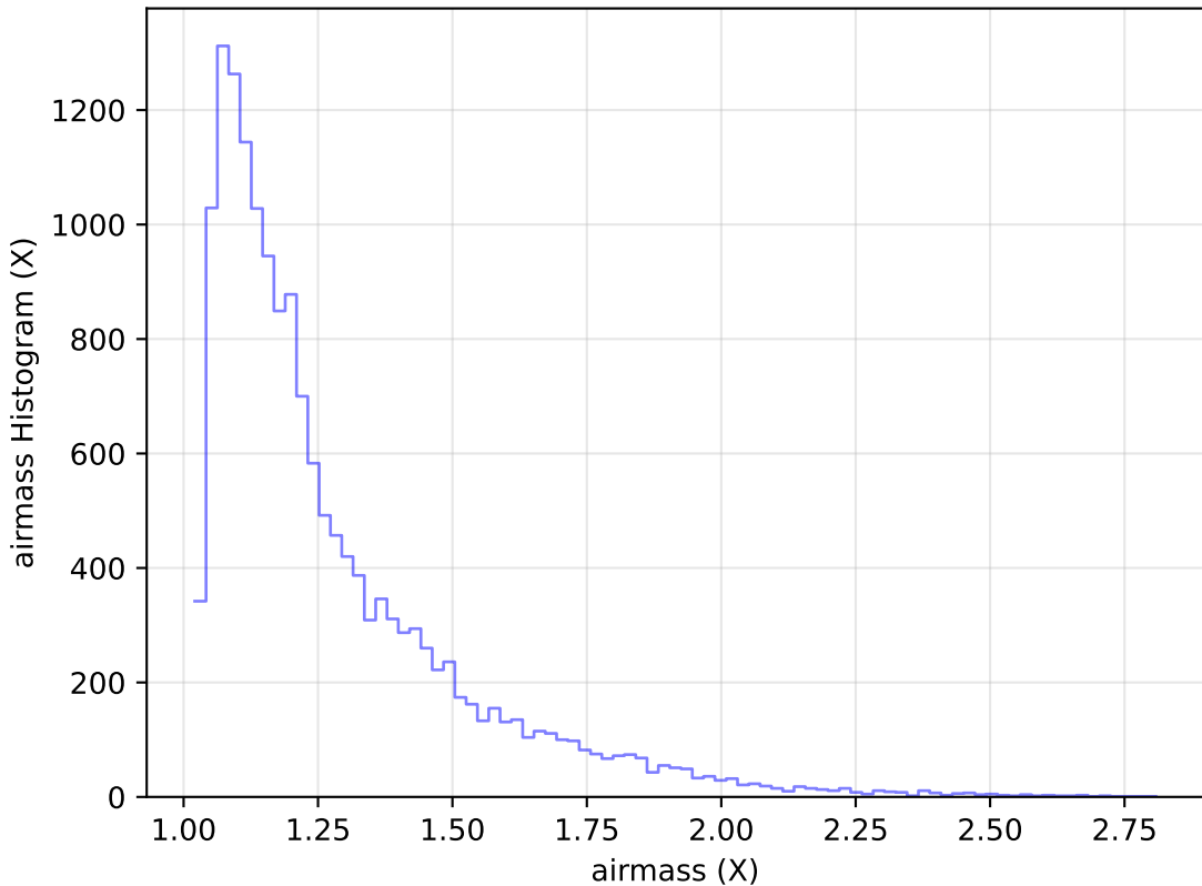
too_elab_r16_d2_griz_v3.4_10yrs Yr 1 u band: airmass Histogram
