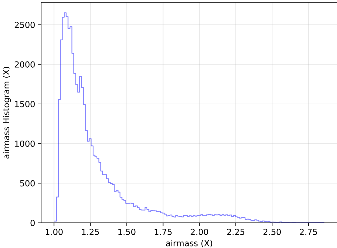
too_elab_r16_d2_griz_v3.4_10yrs Yr 1 r band: airmass Histogram
