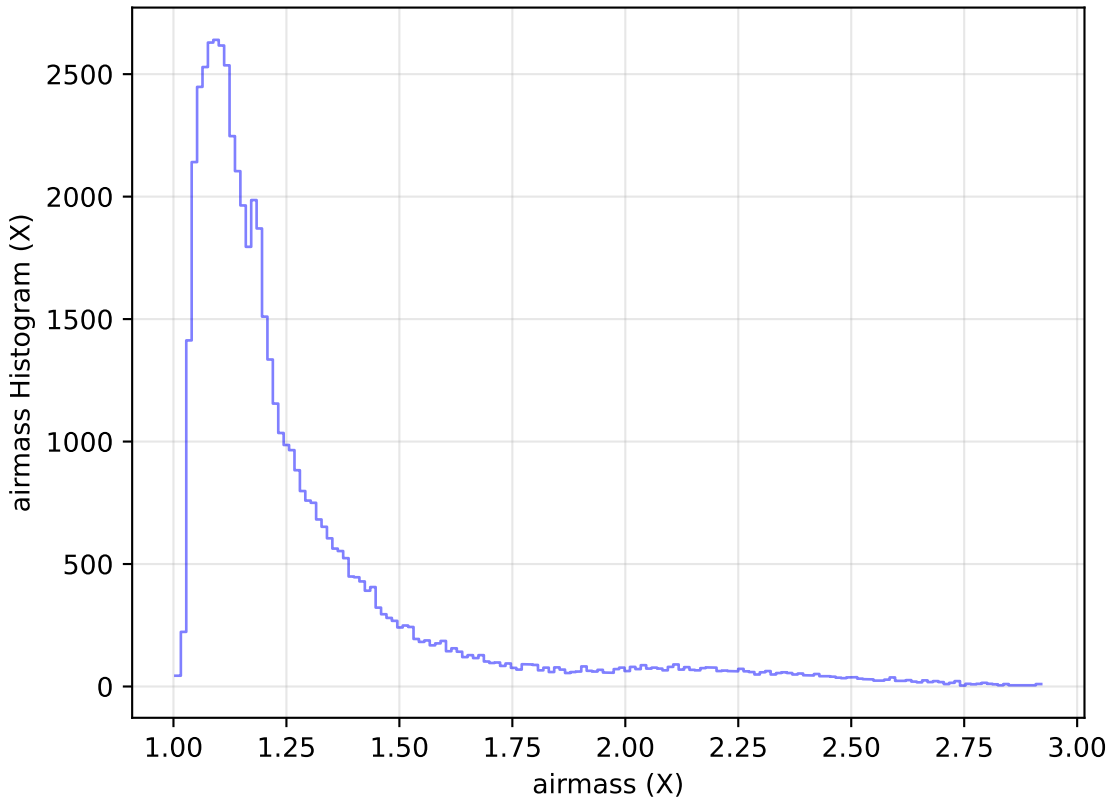
too_elab_r16_d2_griz_v3.4_10yrs Yr 1 i band: airmass Histogram
