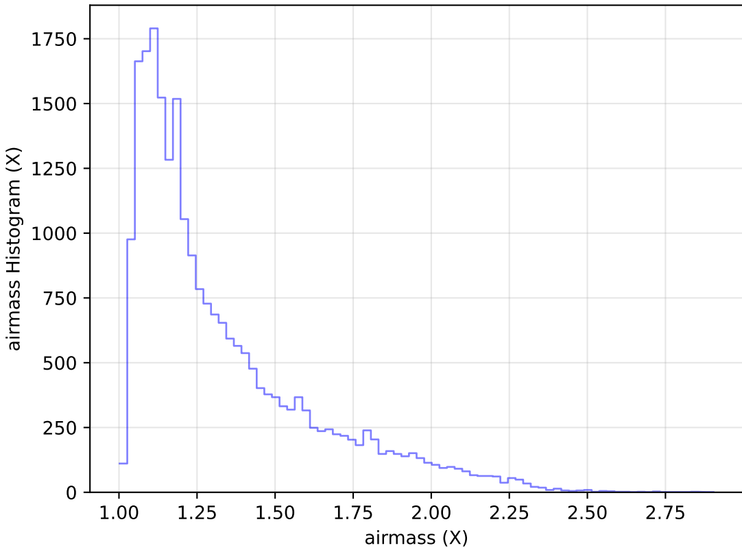
too_elab_r16_d2_griz_v3.4_10yrs Yr 1 g band: airmass Histogram
