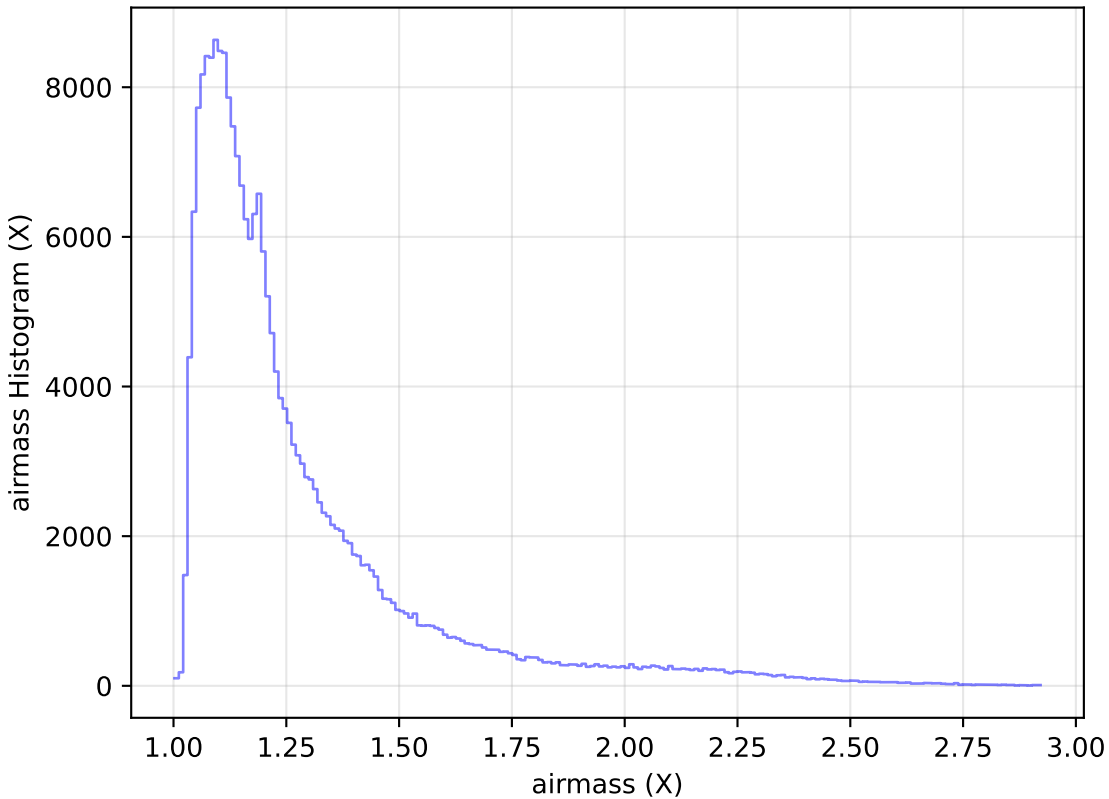
too_elab_r16_d2_griz_v3.4_10yrs Yr 1 all bands: airmass Histogram
