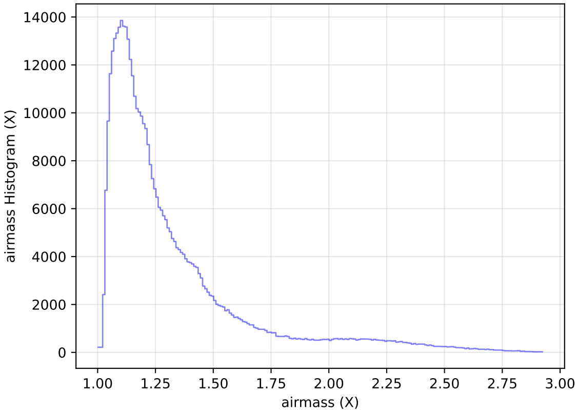
too_elab_r16_d2_griz_v3.4_10yrs WFD z band: airmass Histogram
