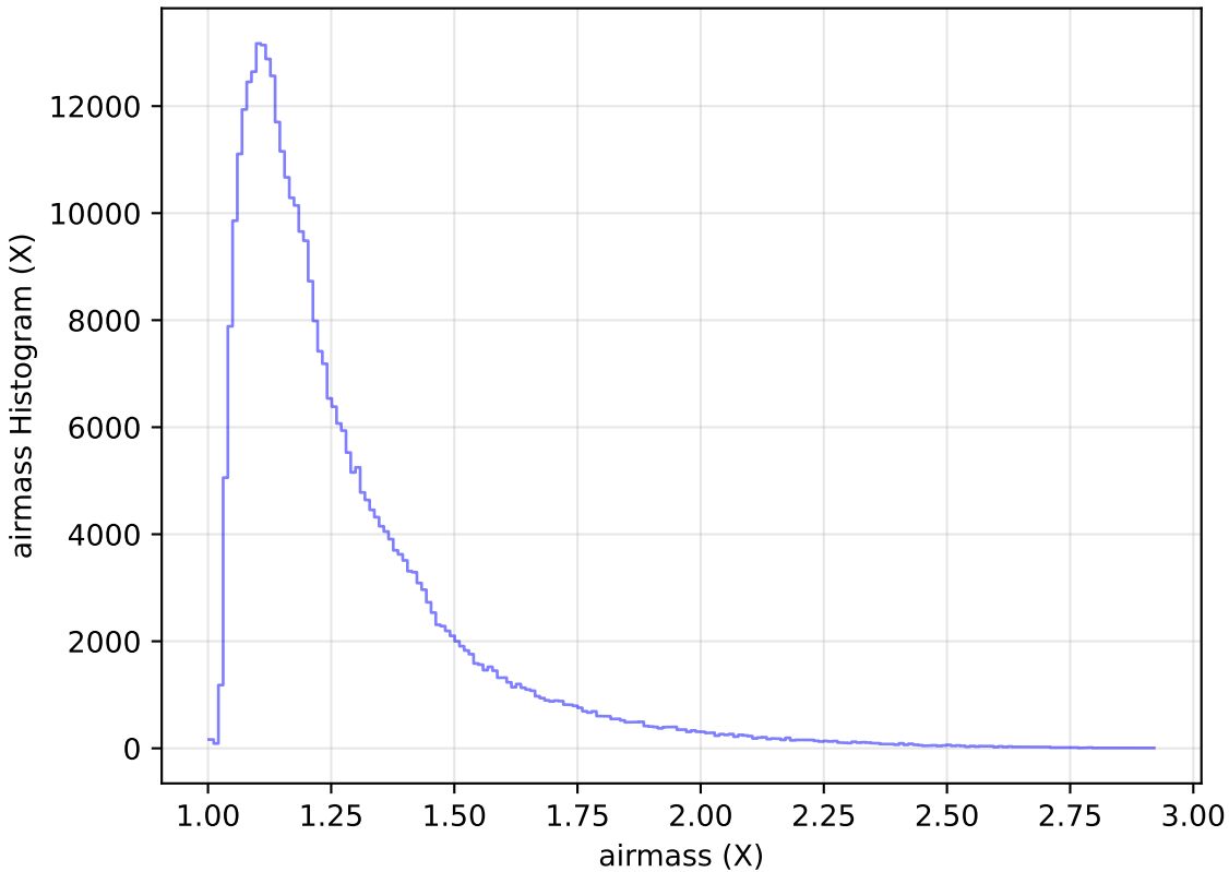
too_elab_r16_d2_griz_v3.4_10yrs WFD y band: airmass Histogram
