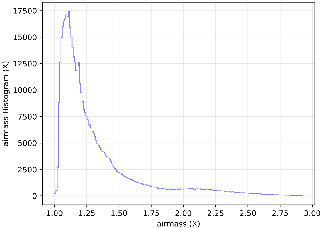
too_elab_r16_d2_griz_v3.4_10yrs WFD i band: airmass Histogram
