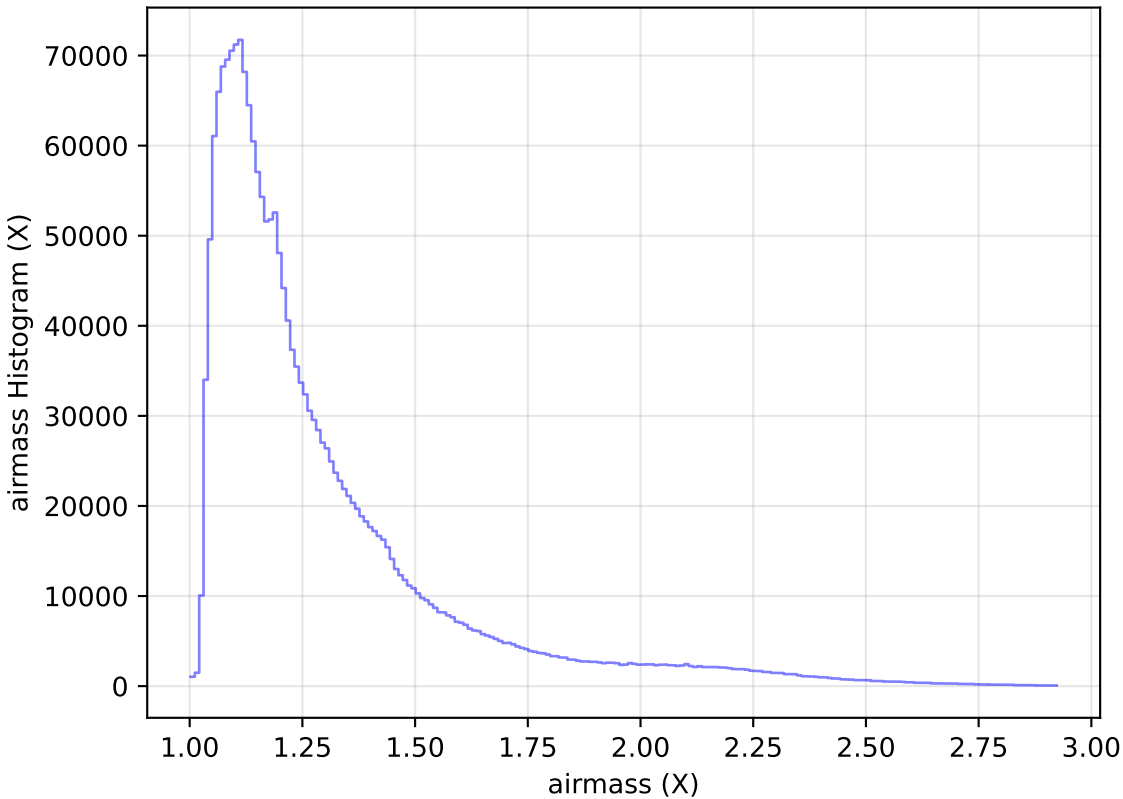
too_elab_r16_d2_griz_v3.4_10yrs WFD all bands: airmass Histogram
