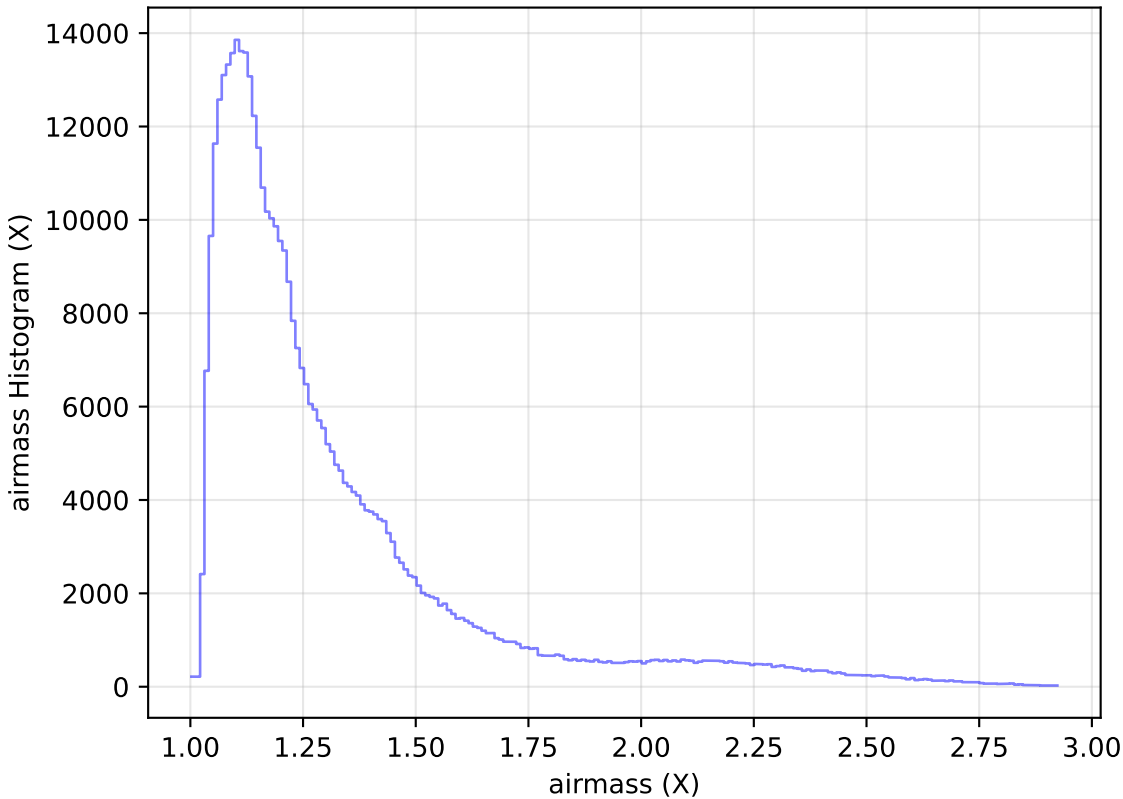
too_elab_r16_d2_griz_v3.4_10yrs All sky z band: airmass Histogram
