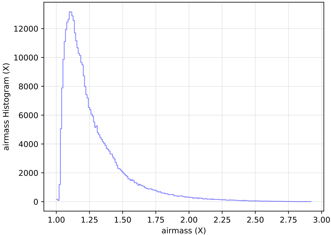
too_elab_r16_d2_griz_v3.4_10yrs All sky y band: airmass Histogram
