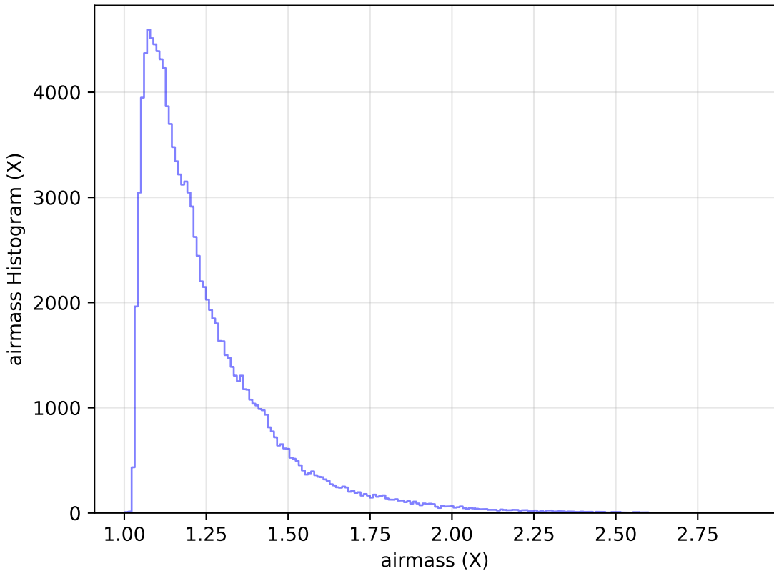
too_elab_r16_d2_griz_v3.4_10yrs All sky u band: airmass Histogram
