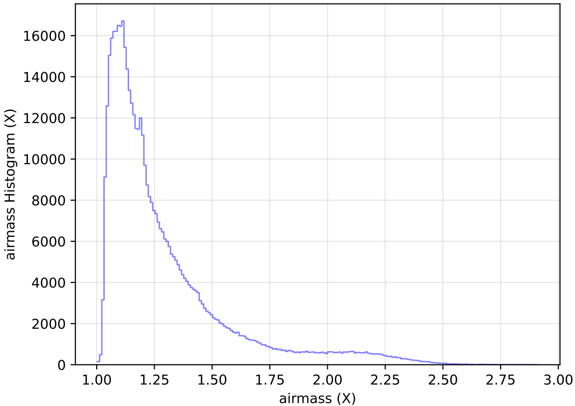
too_elab_r16_d2_griz_v3.4_10yrs All sky r band: airmass Histogram
