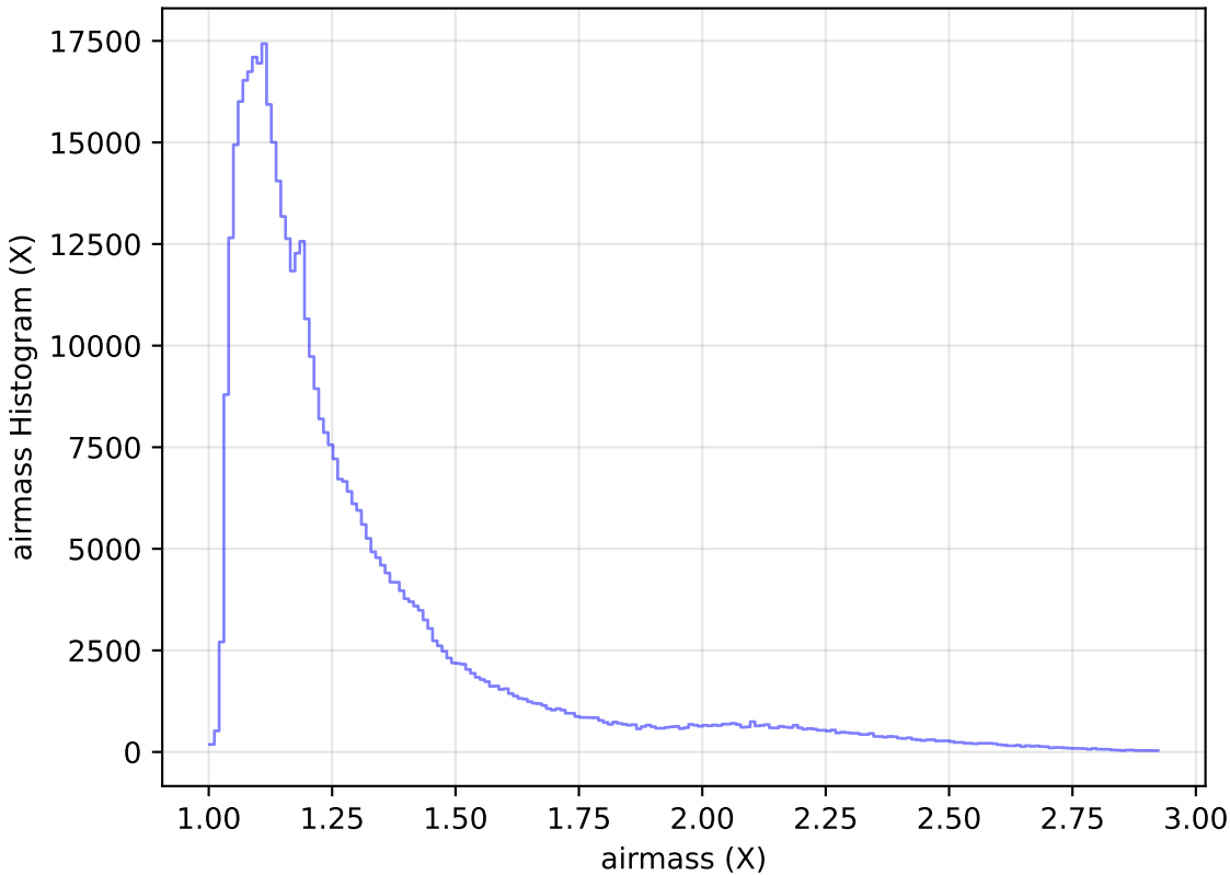
too_elab_r16_d2_griz_v3.4_10yrs All sky i band: airmass Histogram
