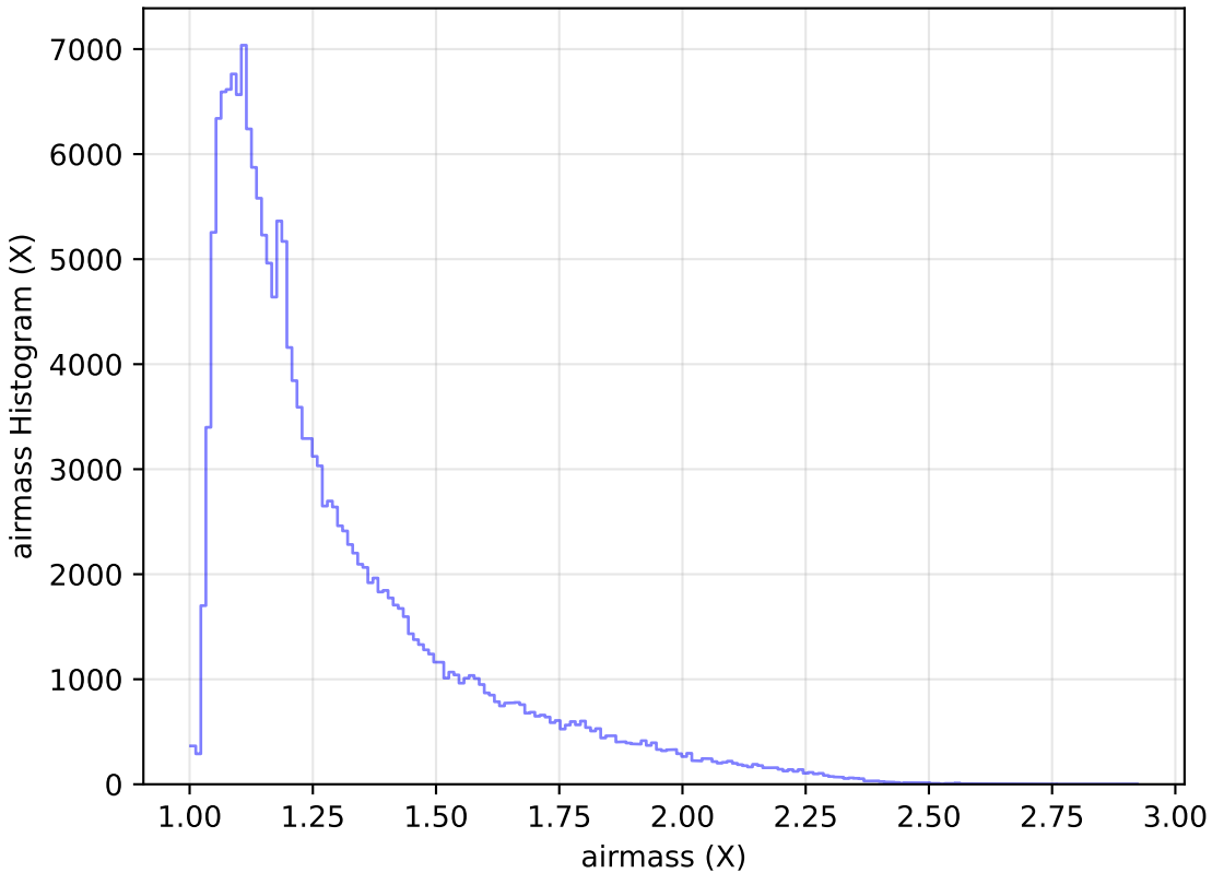
too_elab_r16_d2_griz_v3.4_10yrs All sky g band: airmass Histogram
