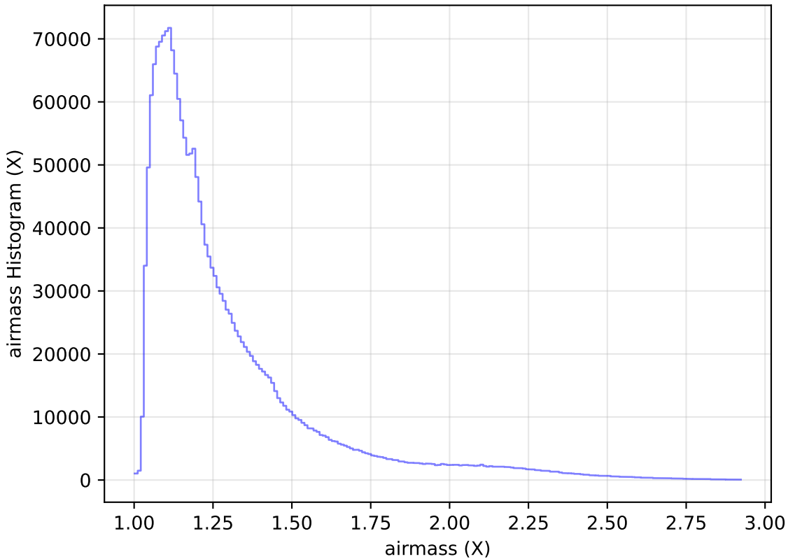
too_elab_r16_d2_griz_v3.4_10yrs All sky all bands: airmass Histogram
