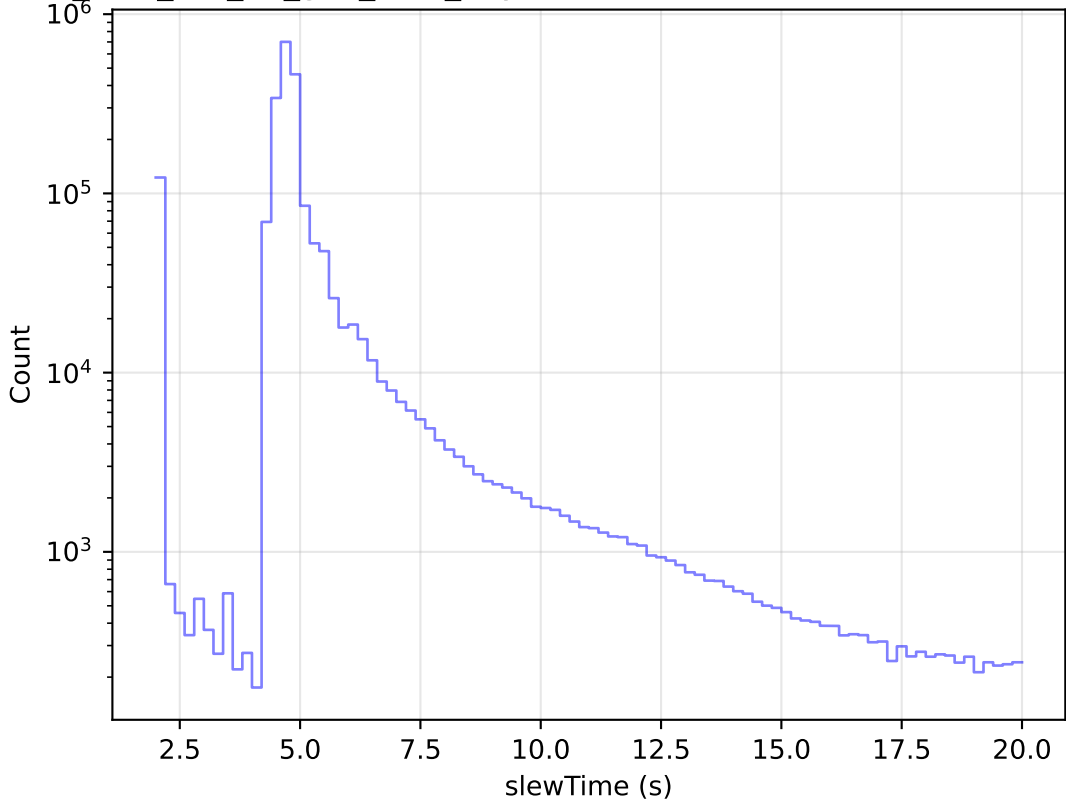
too_elab_r16_d2_griz_v3.4_10yrs All visits: Zoom Slew Time Histogram
