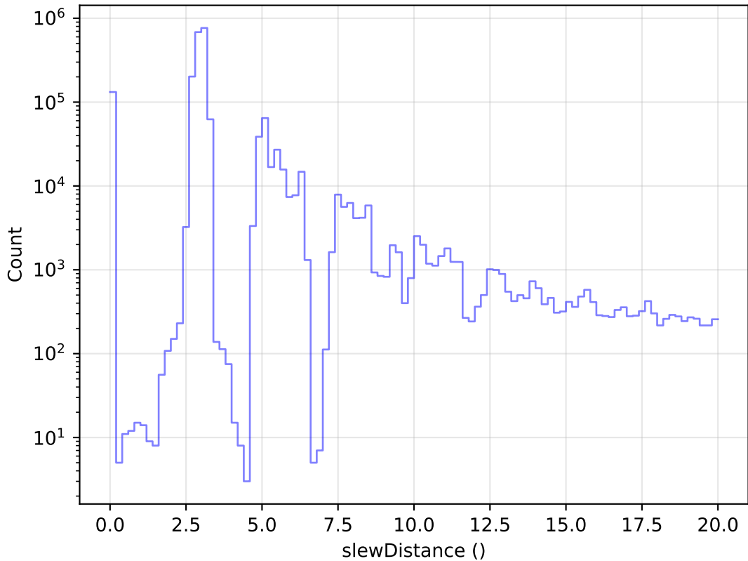
too_elab_r16_d2_griz_v3.4_10yrs All visits: Zoom Slew Distance Histogram
