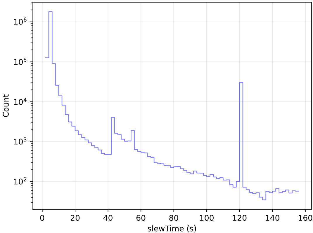
too_elab_r16_d2_griz_v3.4_10yrs All visits: Slew Time Histogram
