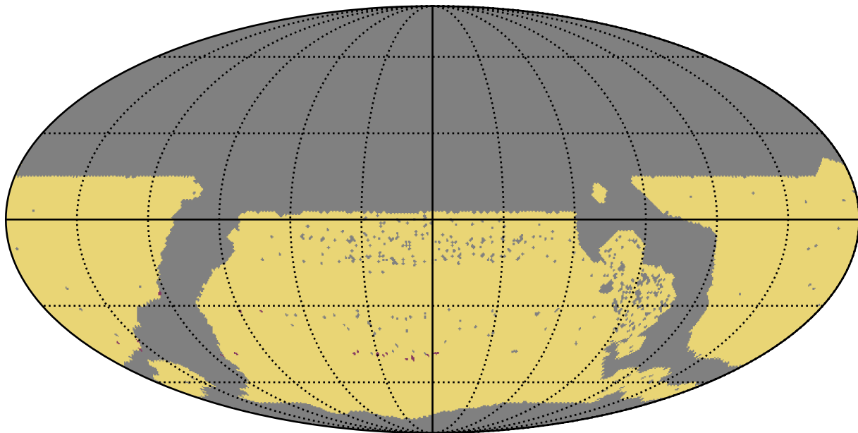
too_elab_r16_d2_griz_v3.4_10yrs WFD: RapidRevisits
