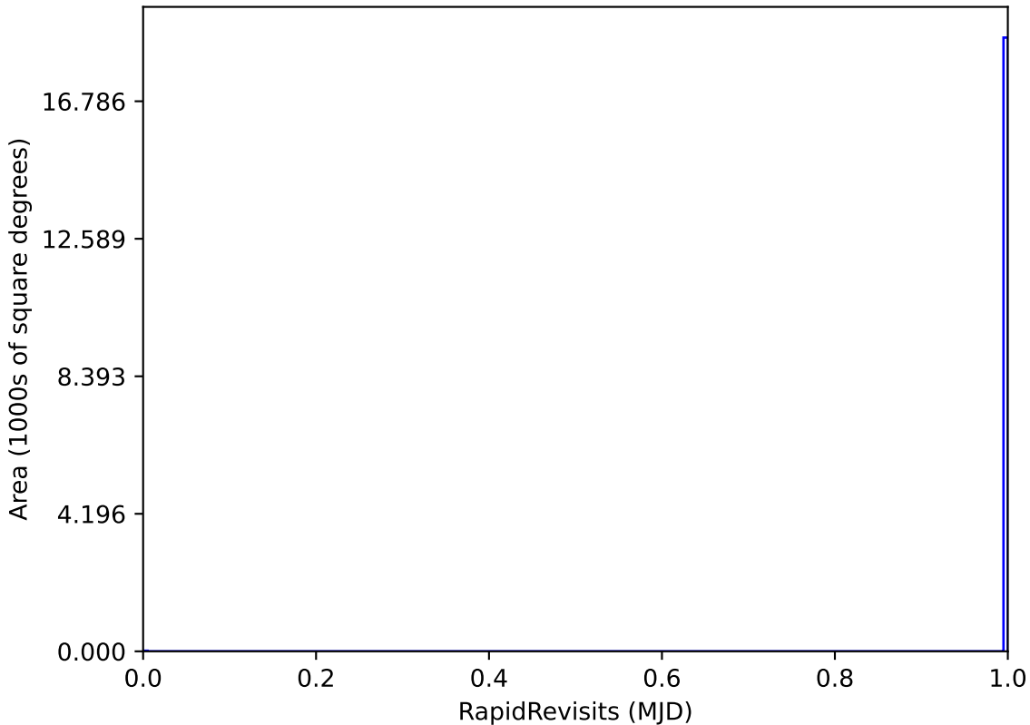
too_elab_r16_d2_griz_v3.4_10yrs WFD: RapidRevisits
