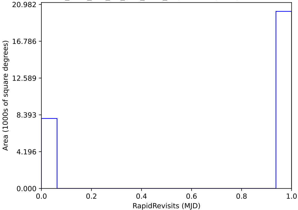
too_elab_r16_d2_griz_v3.4_10yrs All sky: RapidRevisits
