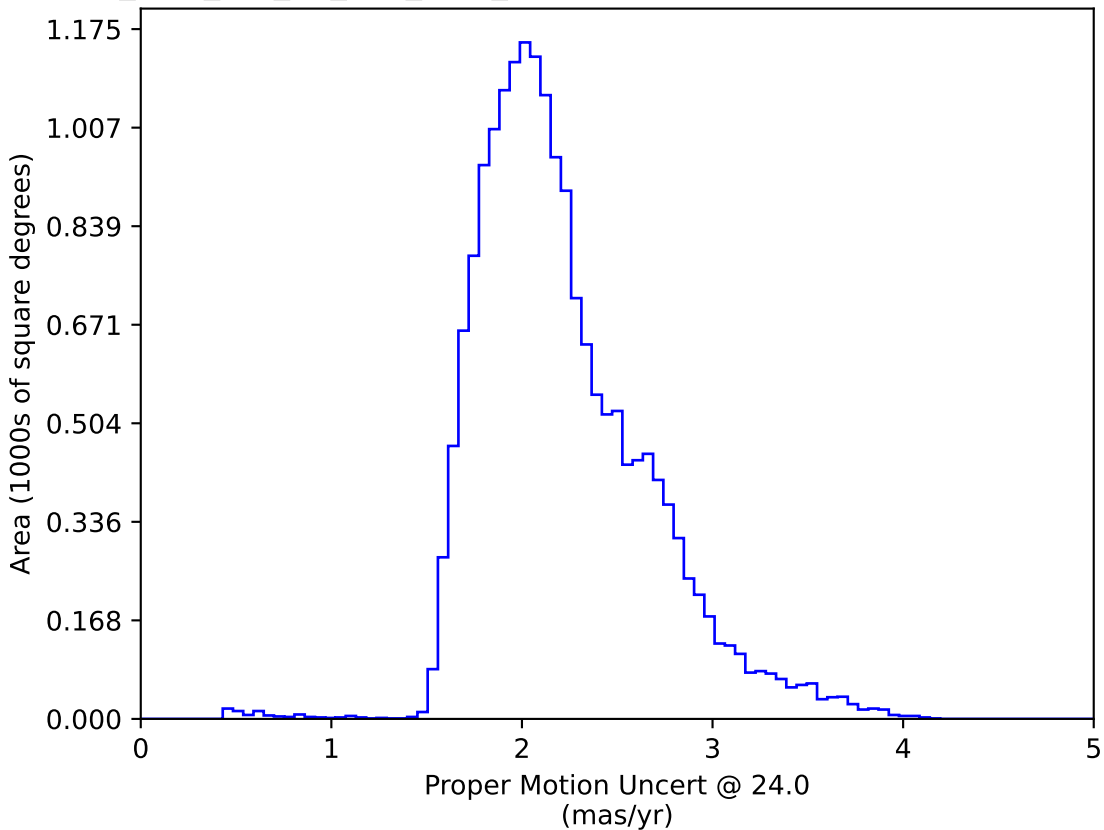
too_elab_r16_d2_griz_v3.4_10yrs WFD: Proper Motion Uncert @ 24.0
