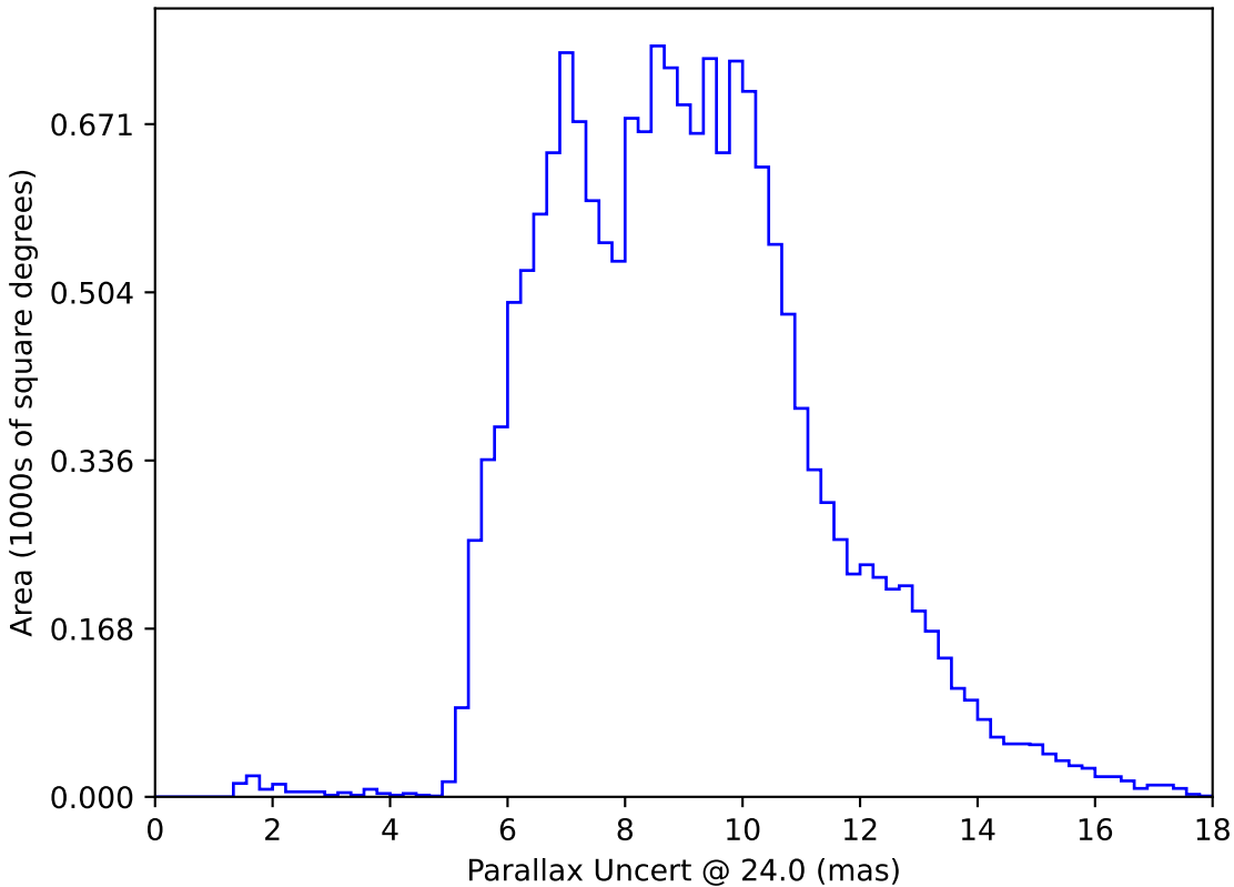
too_elab_r16_d2_griz_v3.4_10yrs WFD: Parallax Uncert @ 24.0
