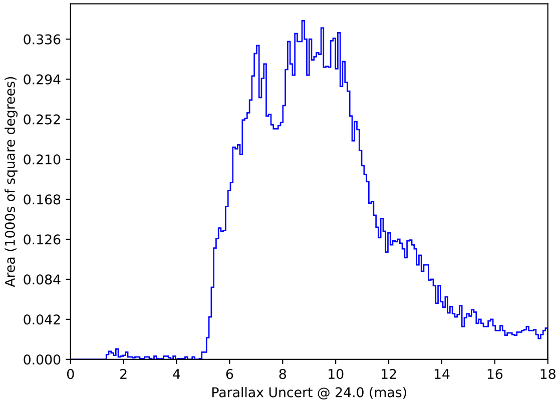
too_elab_r16_d2_griz_v3.4_10yrs All sky: Parallax Uncert @ 24.0
