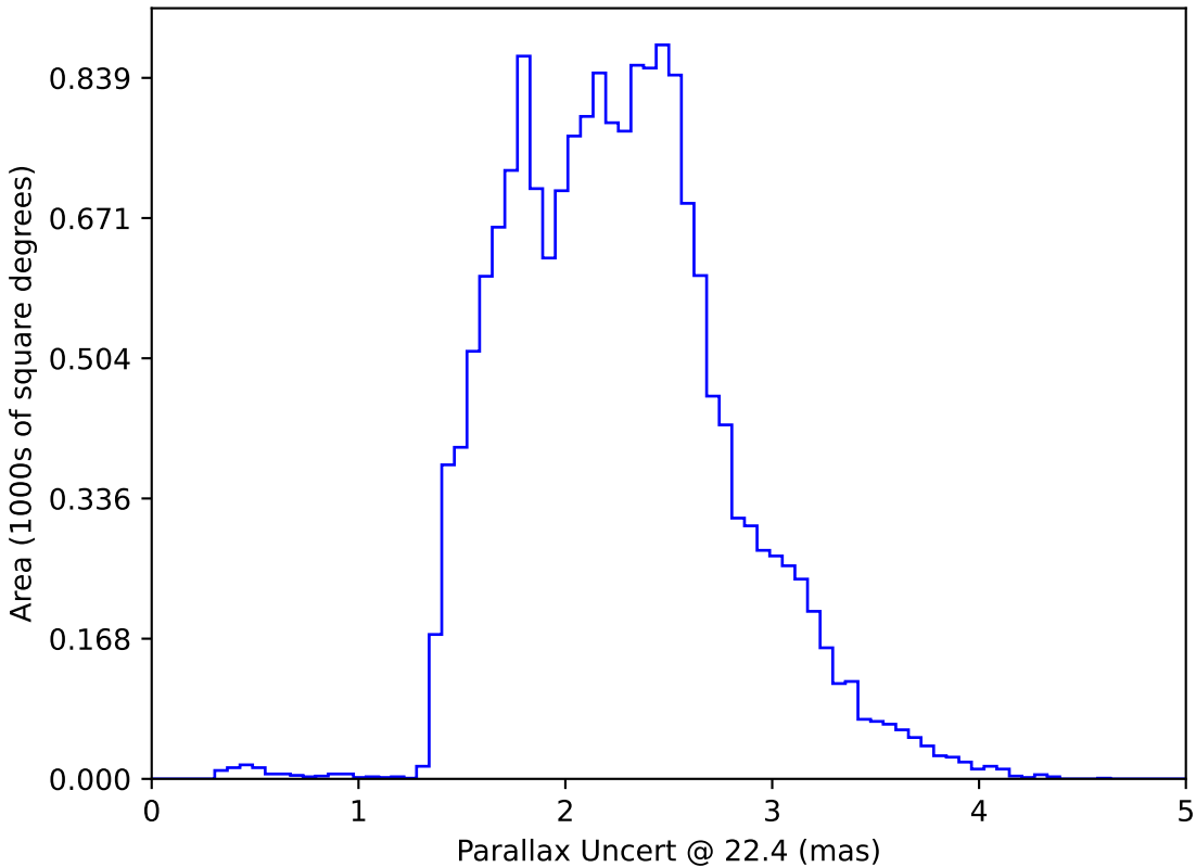
too_elab_r16_d2_griz_v3.4_10yrs WFD: Parallax Uncert @ 22.4
