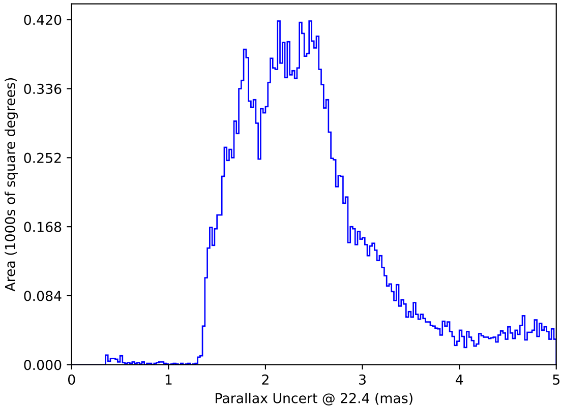
too_elab_r16_d2_griz_v3.4_10yrs All sky: Parallax Uncert @ 22.4
