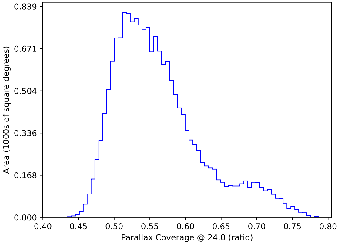
too_elab_r16_d2_griz_v3.4_10yrs WFD: Parallax Coverage @ 24.0
