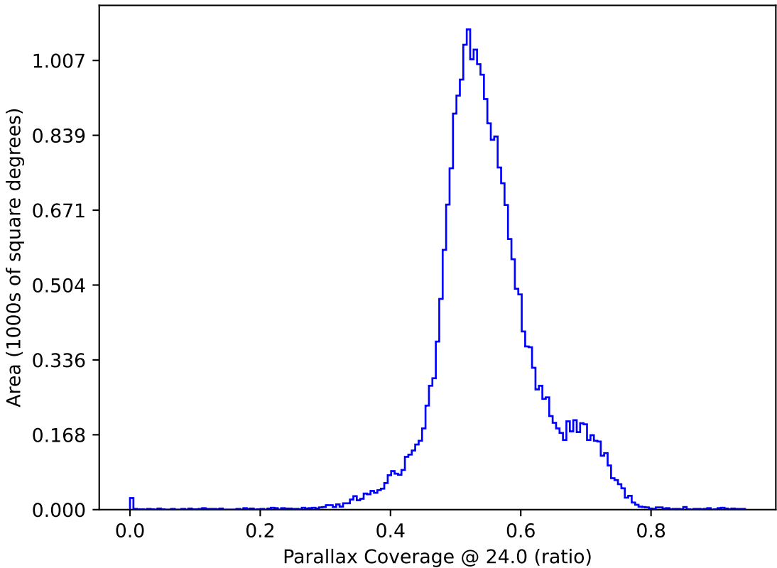
too_elab_r16_d2_griz_v3.4_10yrs All sky: Parallax Coverage @ 24.0
