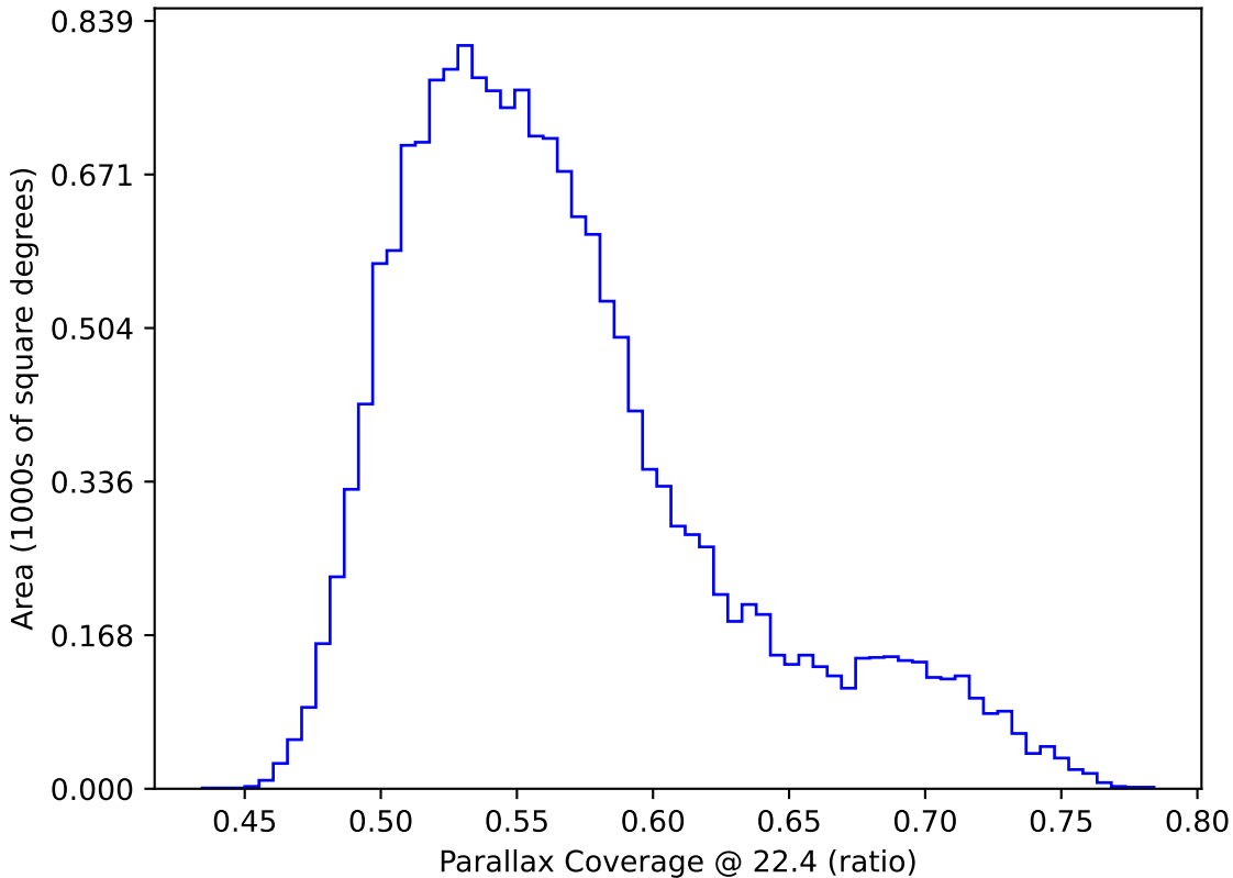
too_elab_r16_d2_griz_v3.4_10yrs WFD: Parallax Coverage @ 22.4
