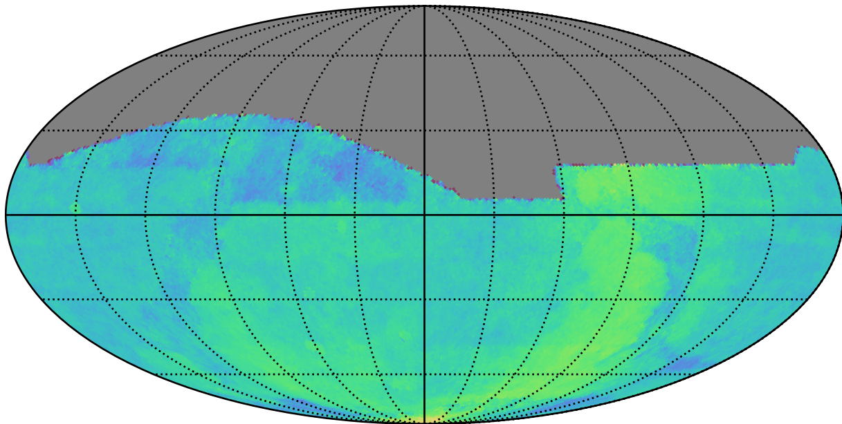
too_elab_r16_d2_griz_v3.4_10yrs All sky: Parallax Coverage @ 22.4
