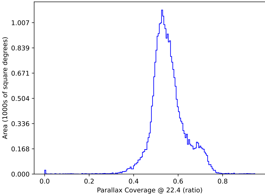
too_elab_r16_d2_griz_v3.4_10yrs All sky: Parallax Coverage @ 22.4
