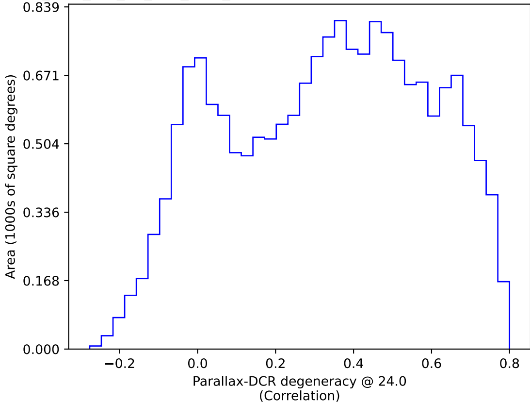
too_elab_r16_d2_griz_v3.4_10yrs WFD: Parallax-DCR degeneracy @ 24.0
