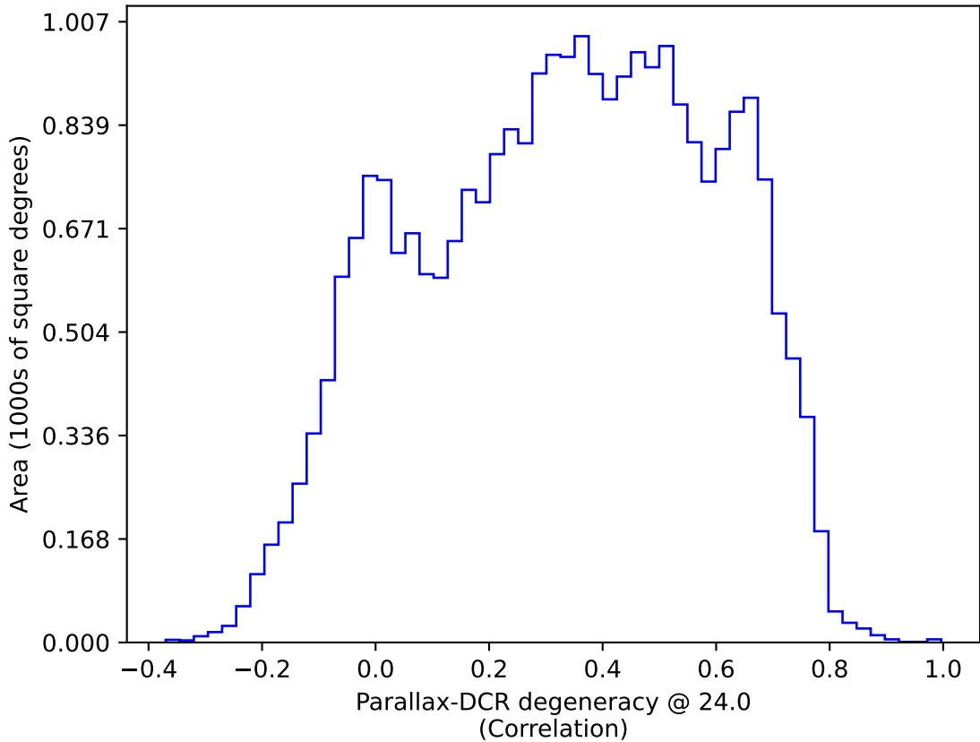
too_elab_r16_d2_griz_v3.4_10yrs All sky: Parallax-DCR degeneracy @ 24.0
