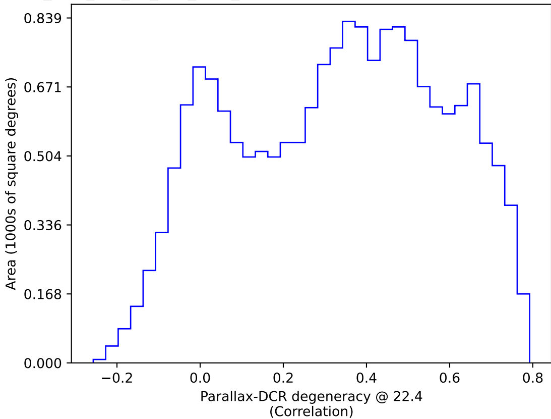
too_elab_r16_d2_griz_v3.4_10yrs WFD: Parallax-DCR degeneracy @ 22.4
