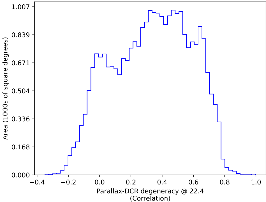
too_elab_r16_d2_griz_v3.4_10yrs All sky: Parallax-DCR degeneracy @ 22.4
