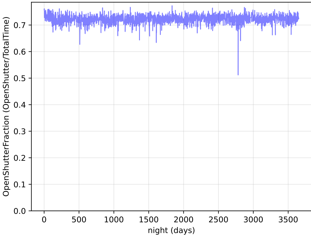
too_elab_r16_d2_griz_v3.4_10yrs Per night: OpenShutterFraction
