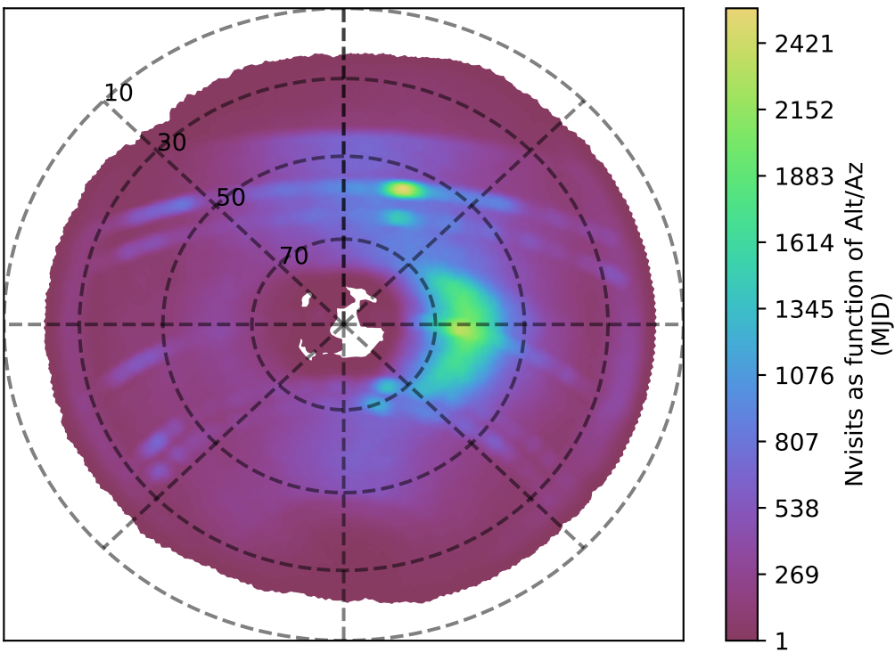
too_elab_r16_d2_griz_v3.4_10yrs z band: Nvisits as function of Alt/Az
