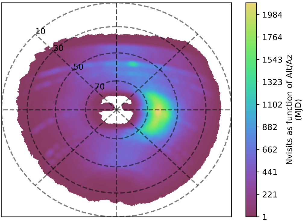
too_elab_r16_d2_griz_v3.4_10yrs y band: Nvisits as function of Alt/Az
